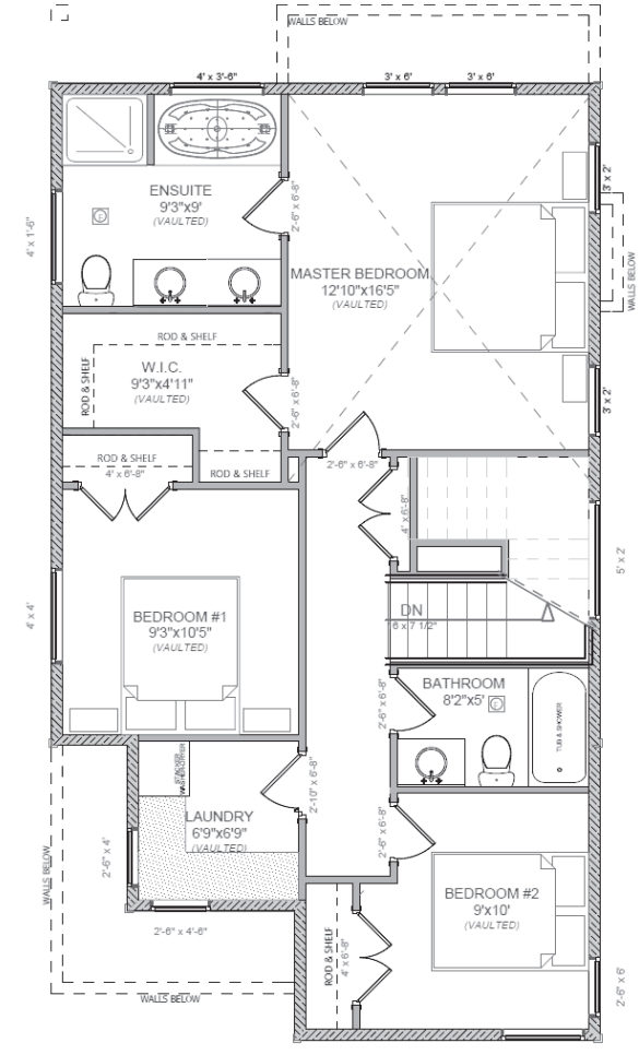
UPPER FLOOR
