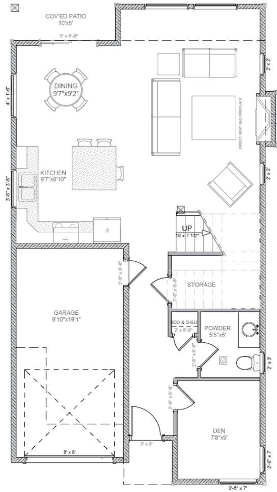
MAIN FLOOR
